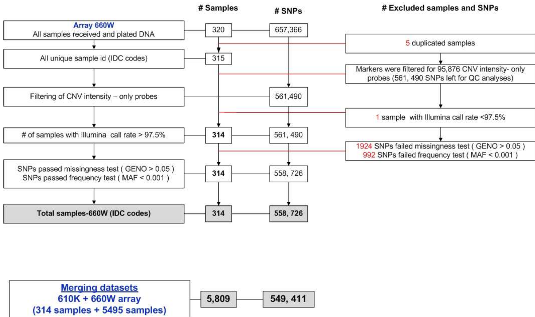
Online Resource 2. Flowchart overview of the Generation R-2 set and merging of the two datasets. Quality control of samples collected at 6 years from peripheral blood (Generation R-2) and processed in platform Illumina HapMap 660-W and merging of the projects. Red font denotes exclusion of either SNPs or samples from the dataset in the different QC steps.
