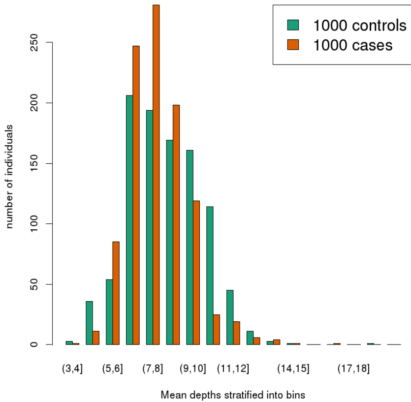
ESM Figure 3 The average depths distribution in 1,000 cases and 1,000 controls after removal of low quality bases.
