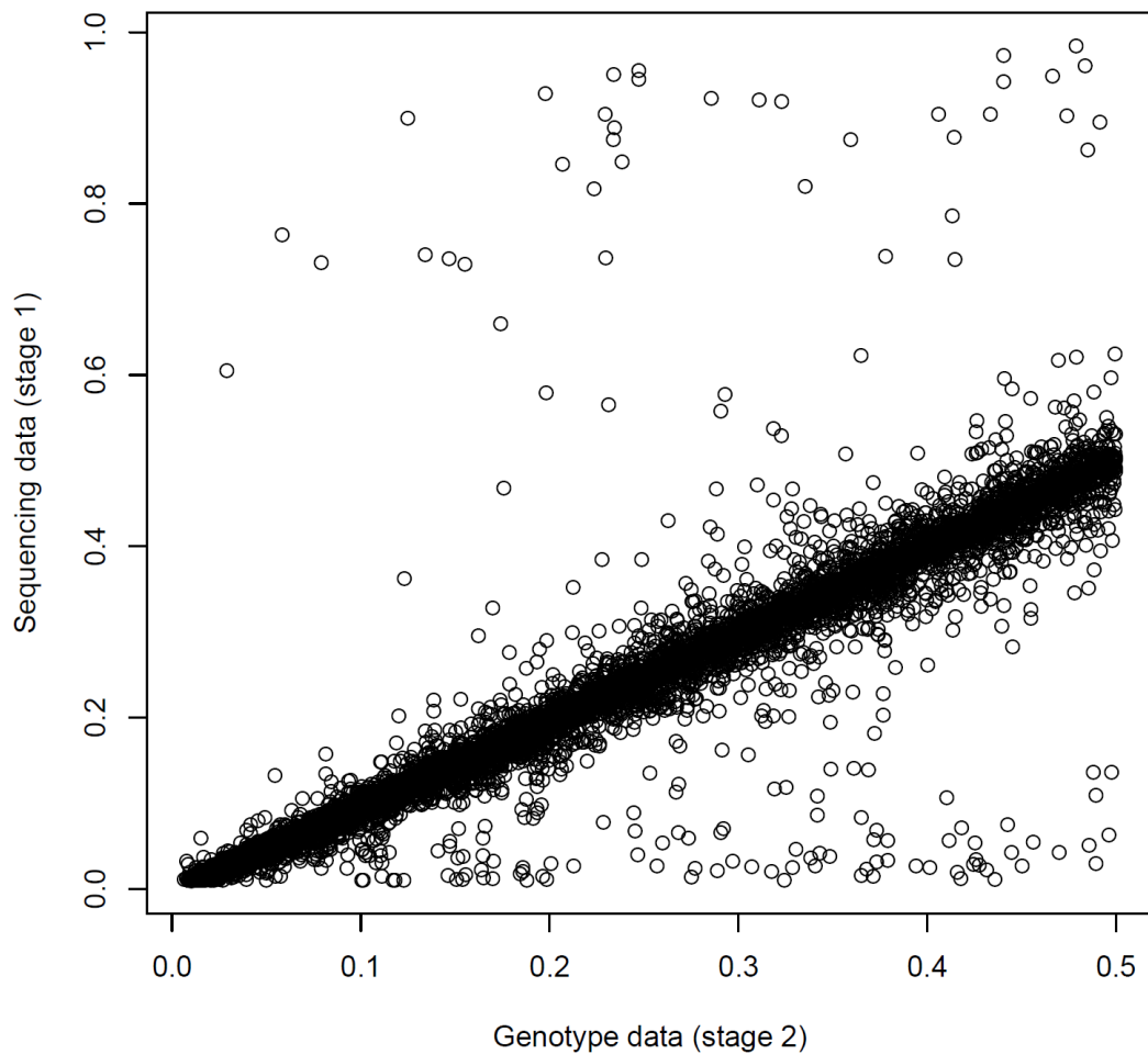
ESM Figure 5 Comparison of allele frequencies from exome sequencing with chip genotyping
