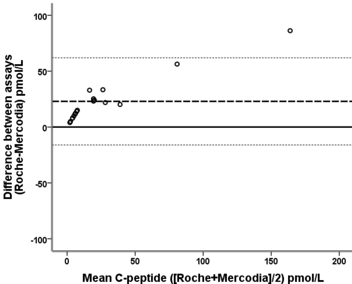
Supplementary figure 1. Bland-Altman plot comparing Roche serum C-peptide electrochemiluminescence assay with Mercodia Ultrasensitive ELISA. Mean difference (standard deviation) was 23 (20) pmol/l
