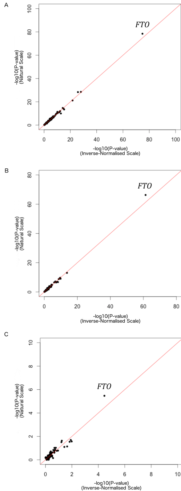
ESM Figure 2. Association statistics for 72 known BMI variants when analysing BMI on an inverse-normalised scale (X axis) compared to its natural (right-hand skewed) scale (Y axis), under (A) additive, (B) recessive and (C) dominance deviation models.
