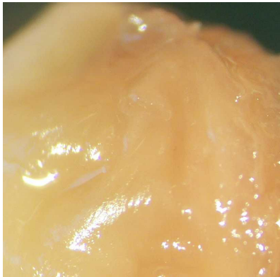
Host FVB
