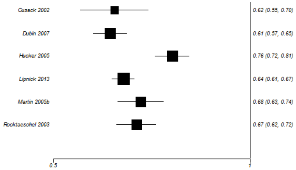
Summary meta-analysis plot [random effects]
