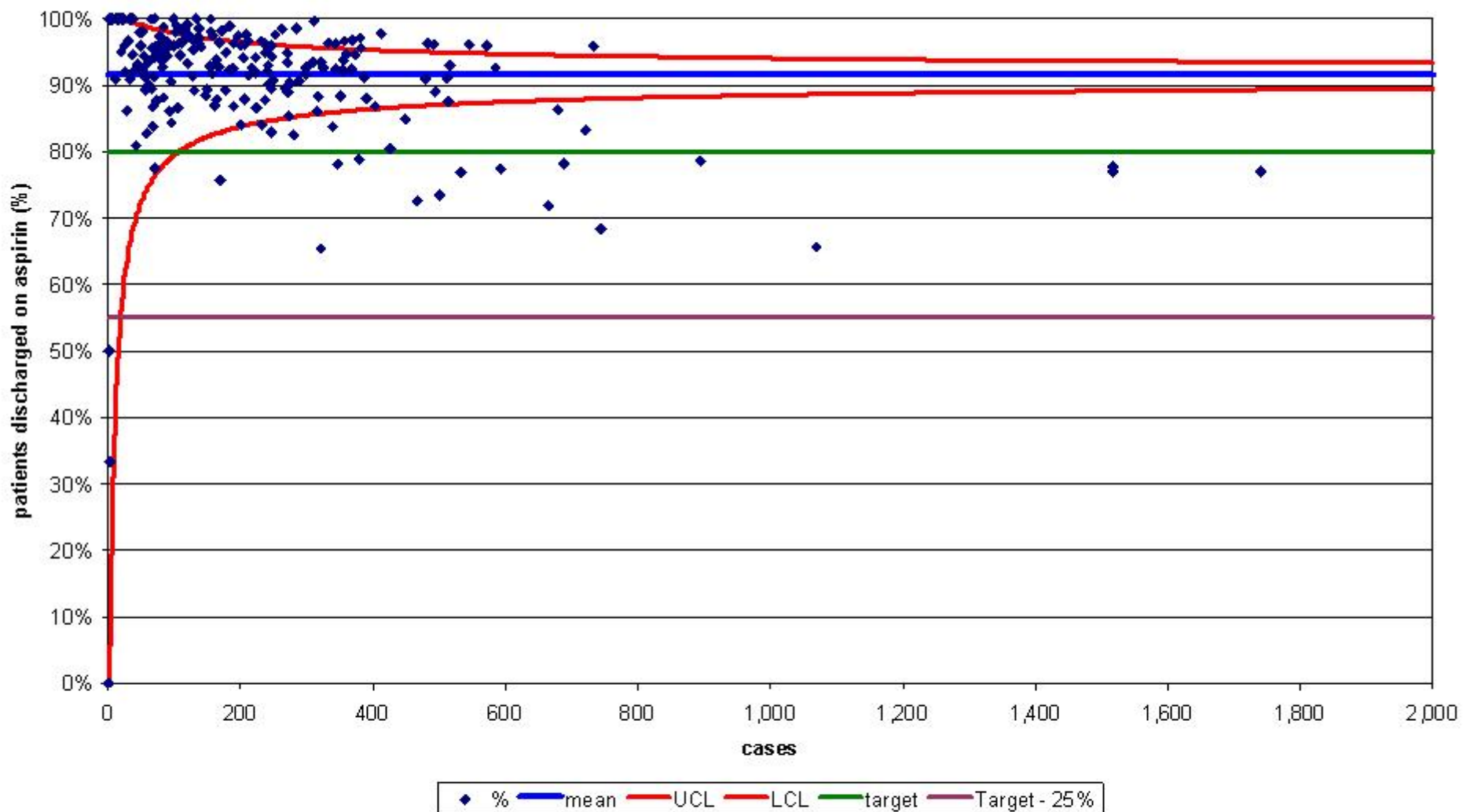
MINAP Secondary prevention medications: patients discharged on aspirin (%)
