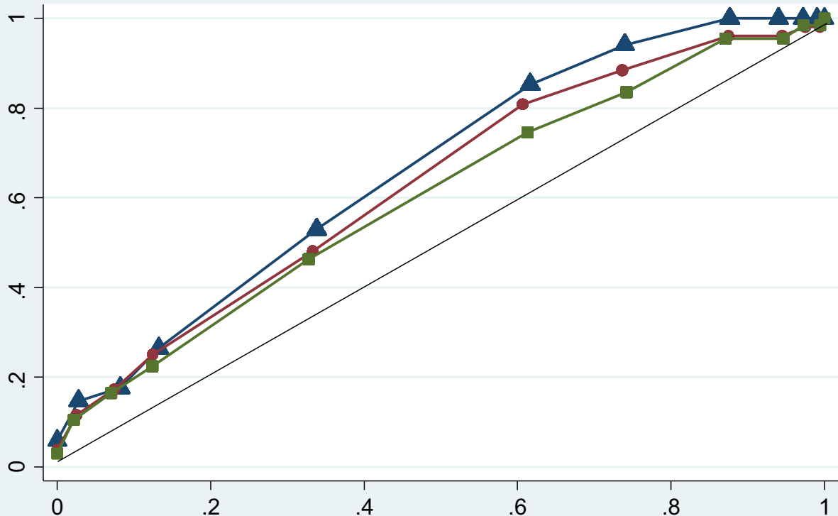
ROC of the LACE index score to predict post discharge ED revisits at 30, 60, and 90 days
