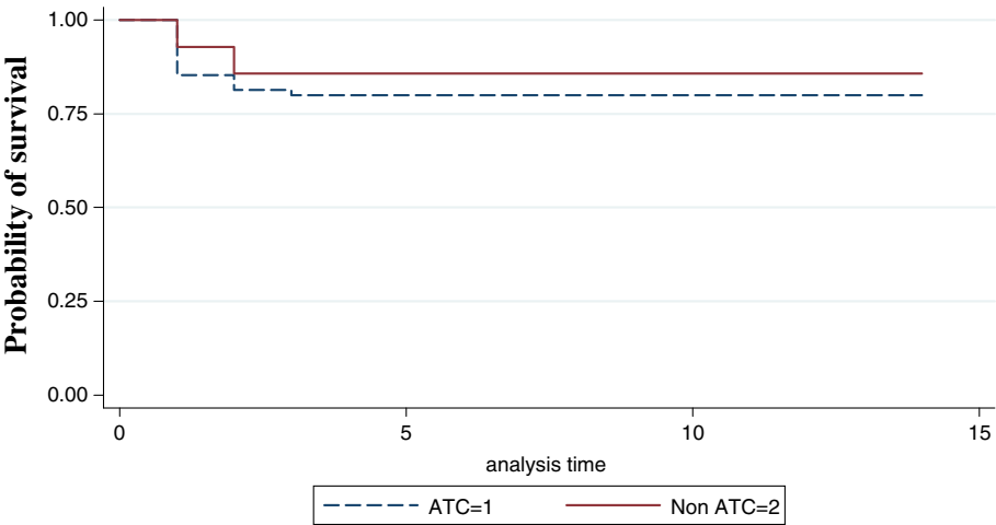
Kaplan-Meier survival estimates for the general population
