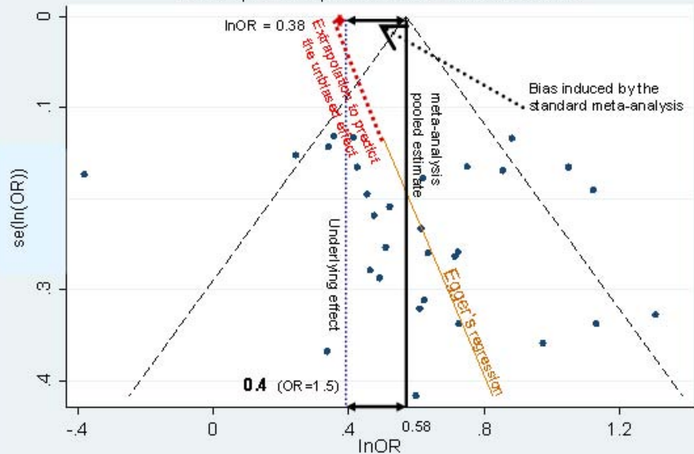
Funnel plot with pseudo 95% confidence limits
