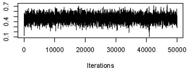
Trace of x.3
