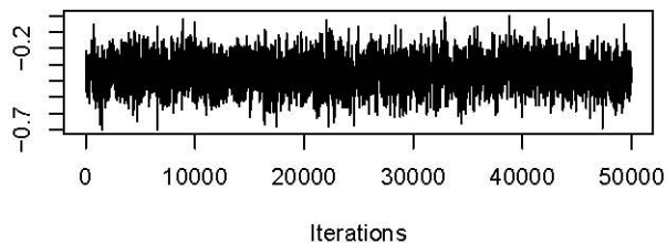
Trace of x.2
