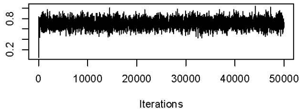
Trace of x.1
