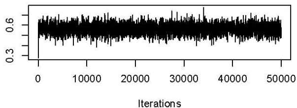
Trace of x.4
