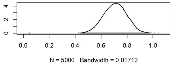
Density of x.1
