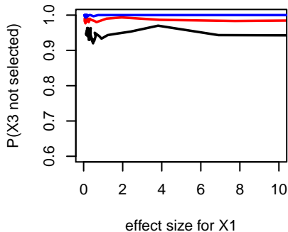
b) Data generating process 3
