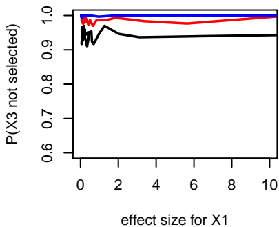
e) Data generating process 5
