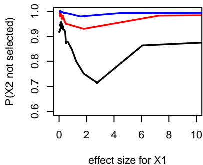
d) Data generating process 4
