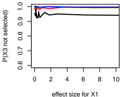
c) Data generating process 4
