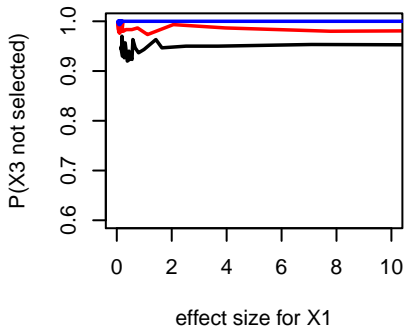
a) Data generating process 2
