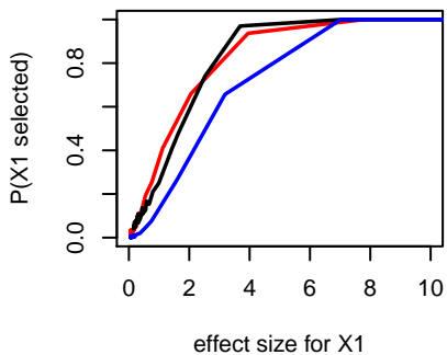
a) Data generating process 2
