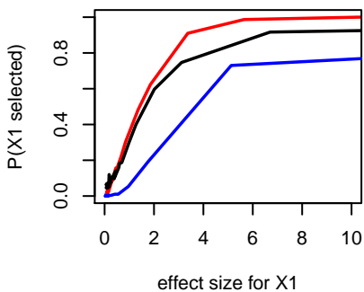
d) Data generating process 5
