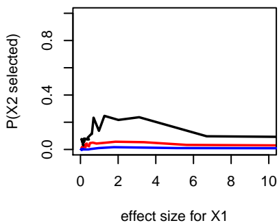
e) Data generating process 5
