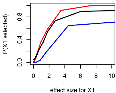
c) Data generating process 4
