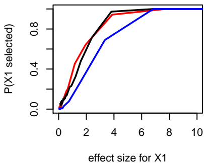
b) Data generating process 3
