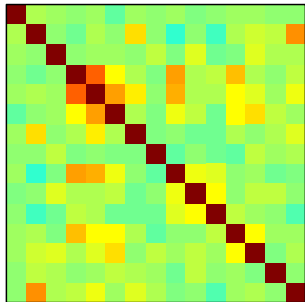
X correlation
