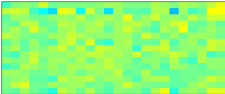
Cross-correlation
