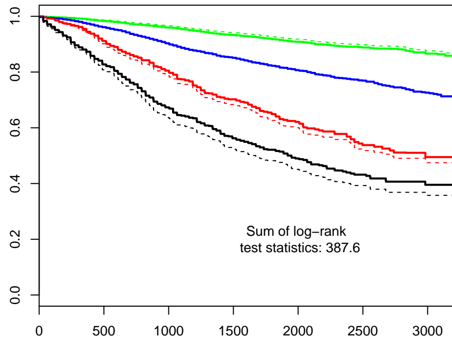
Proportional Sampling
