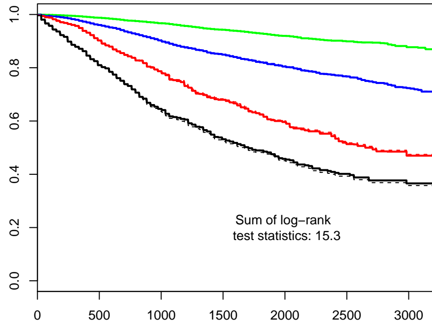
Predictive Mean Matching
