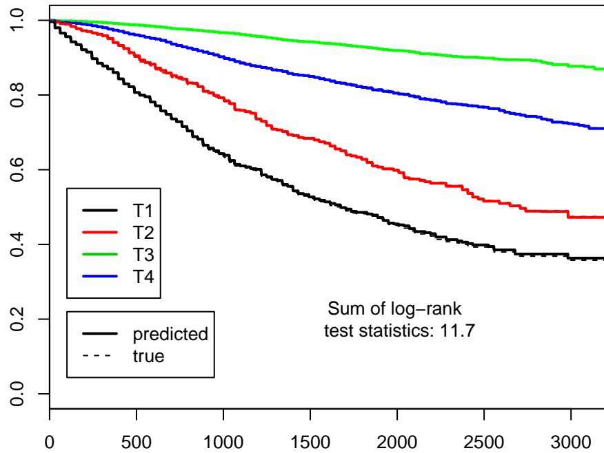
Polytomous Regression
