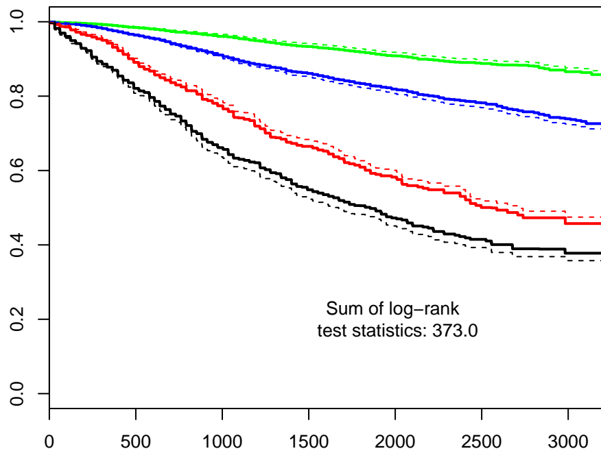
Random Forest
