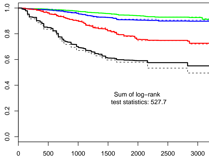
Proportional Sampling
