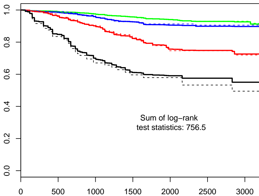
Random Forest
