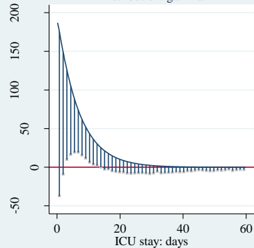
Distribution: gamma
