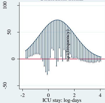
Distribution: normal
