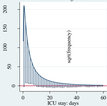
Distribution: lognormal
