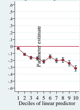
GLM IVG-log: determination
