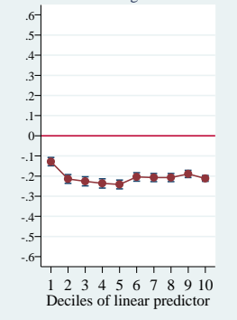
GLM IVG-log: validation
