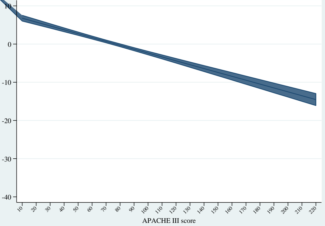
Contrasts of Predictive Margins: OLS, raw-scale
