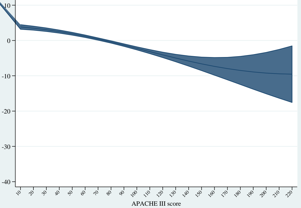
Contrasts of Predictive Margins: GLM log-Gaussian
