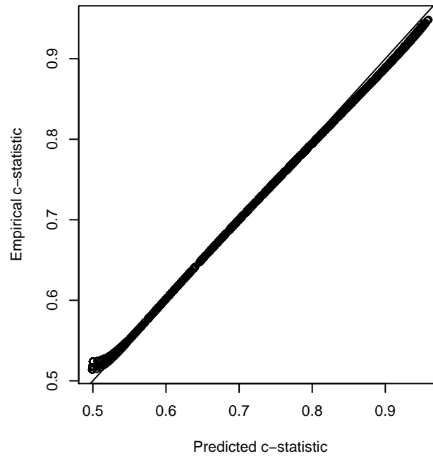
uniform: Predictions using formula (2)
