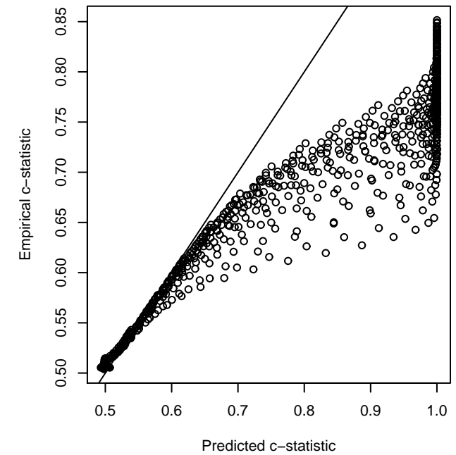
Lognormal: Predictions using formula (1)
