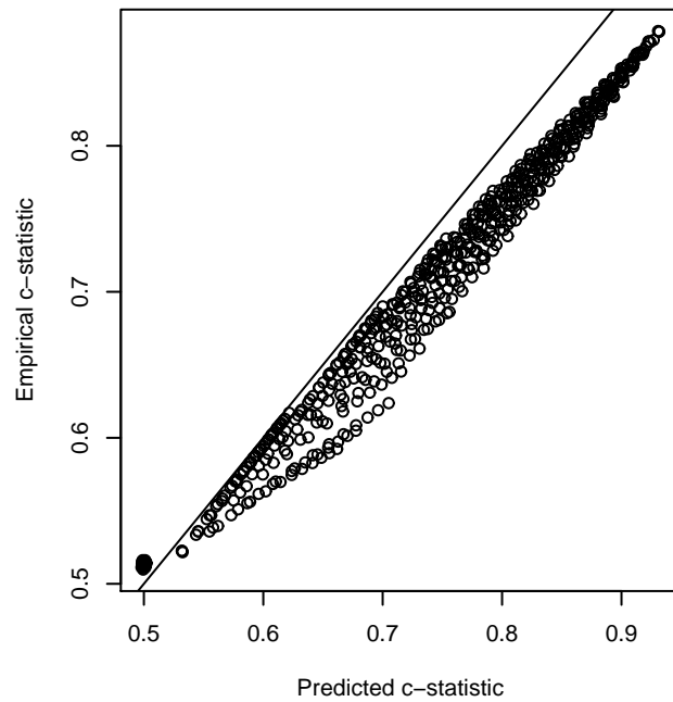
Gamma: Predictions using formula (1)
