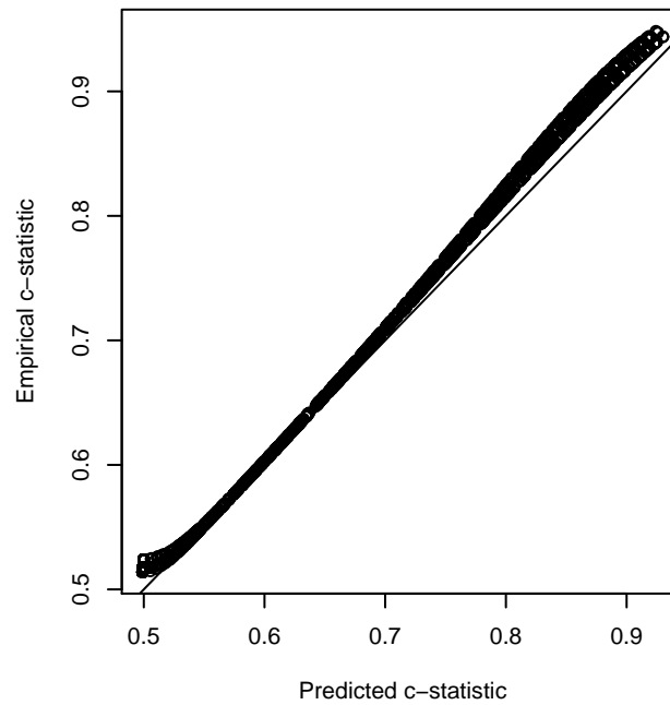
uniform: Predictions using formula (1)
