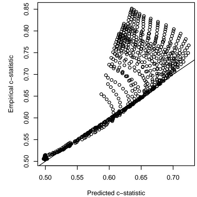
Lognormal: Predictions using formula (2)
