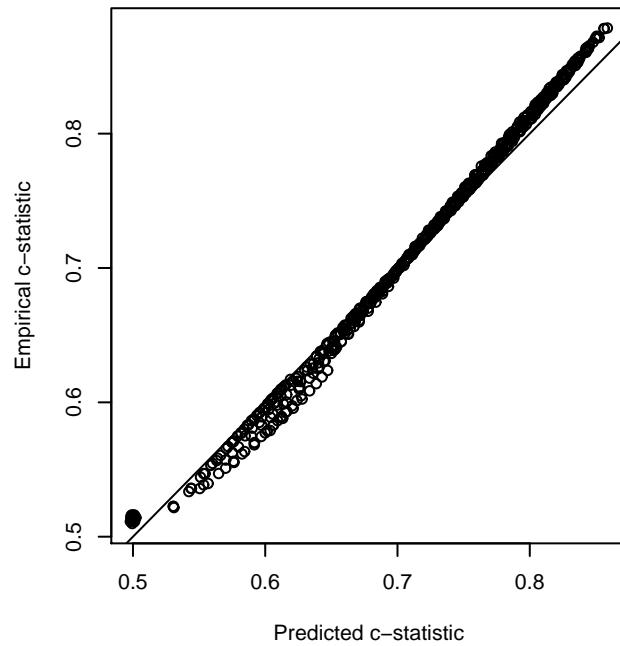
Gamma: Predictions using formula (2)
