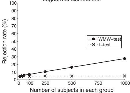
Lognormal distributions
