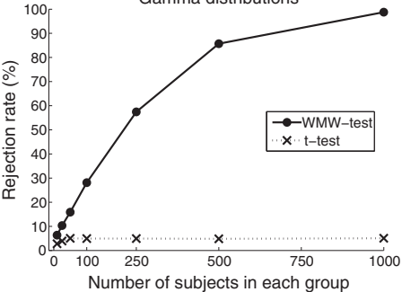
Gamma distributions
