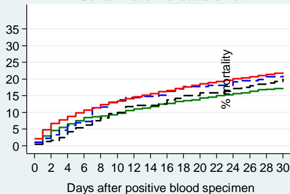
Contamination vs. bacteremia
