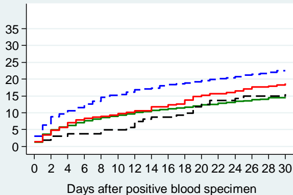
Healthcare- vs. no healthcare-association
