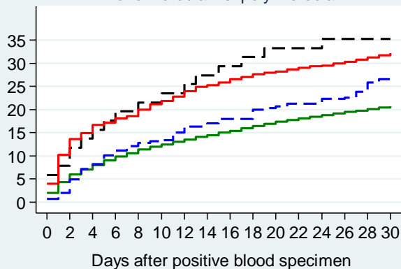
Monomicrobial vs. polymicrobial
