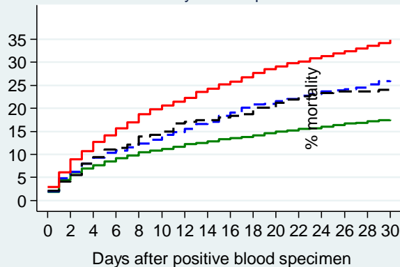
Community- vs. hospital-onset
