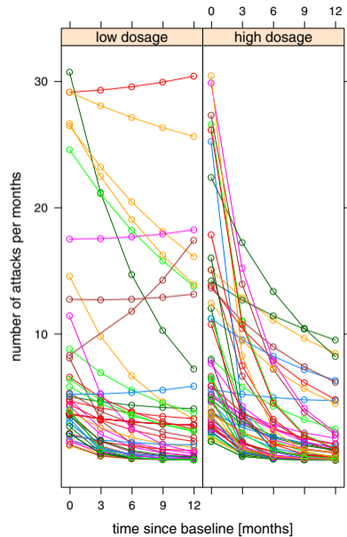
C) Poisson, IS
