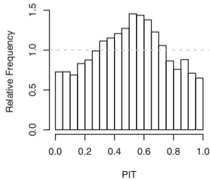
NB, IS
