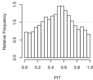
ZIP, IS
