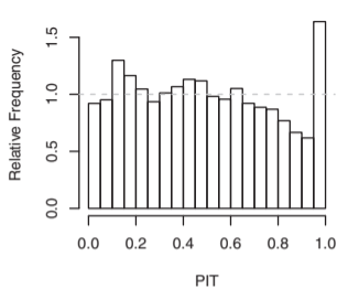
ZIP, I
