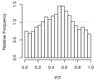
Poisson, IS
