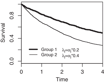
PH- Proportional Hazards
