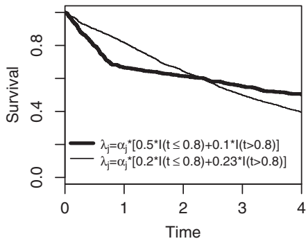
CH- Crossing Hazards
