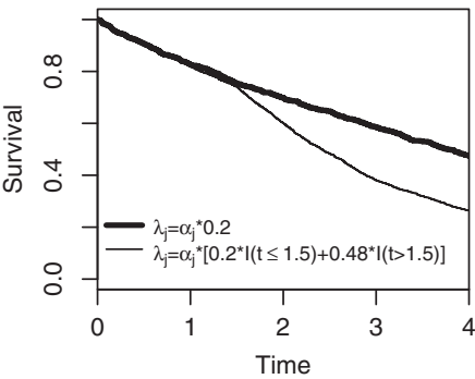
LD- Late Difference
