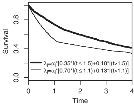
ED- Early Difference
