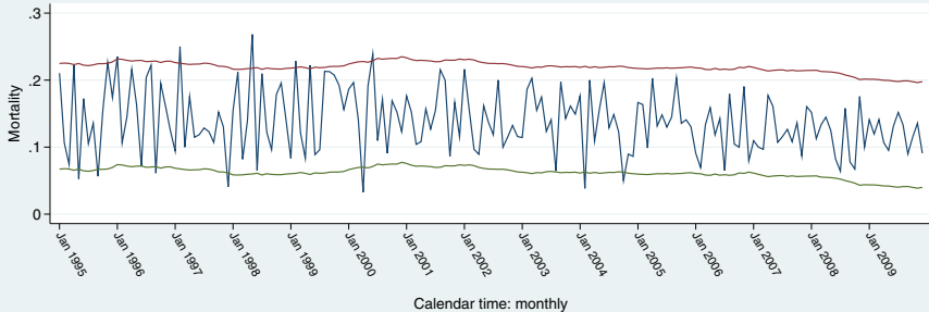
EWMA \lambda = 0.05 for expected mortality (10% increase), fixed control limits for raw mortality
