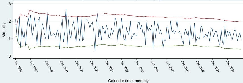
EWMA \lambda = 0.05 for expected mortality (10% increase), time-varying control limits for raw mortality
