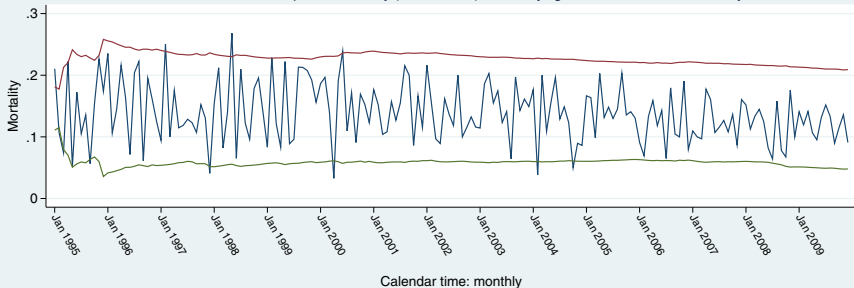
EWMA \lambda = 0.05 for expected mortality (10% increase), time-varying control limits for raw mortality
