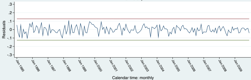
Optimal EWMA fixed control limits for multiplicative seasonal ARMA residuals
