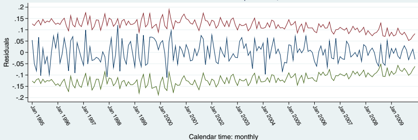
Detrended expected series vs one-setp ARMA predictions, 3SE CL
