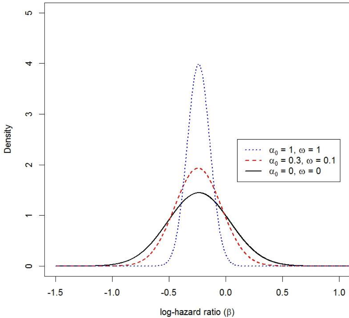
Figure A7: Posterior distribution of the log-hazard ratio depending on the values of the weighting parameters.
