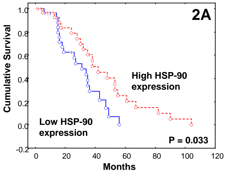
All cases
