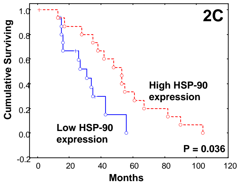
G1/G2 cases
