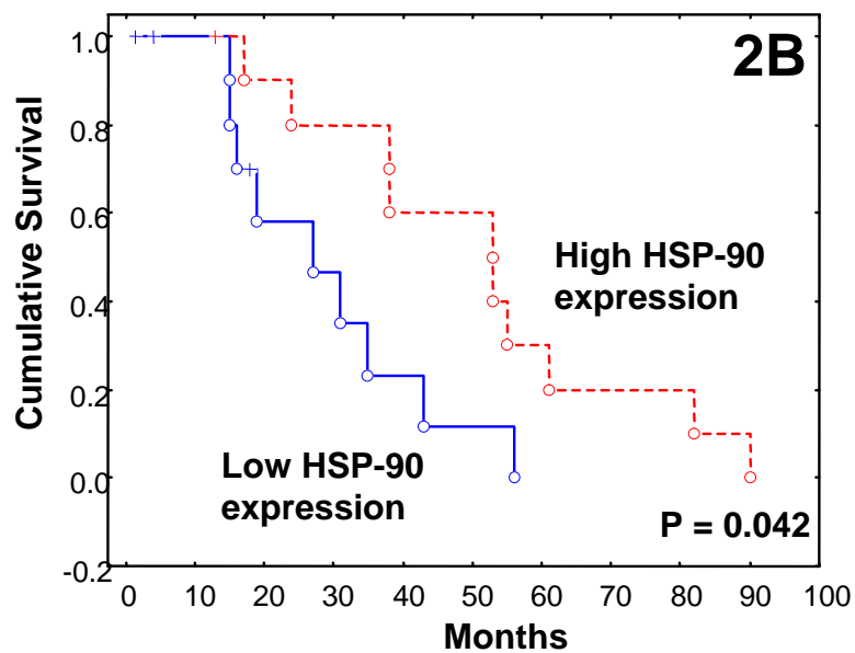
pN0 cases
