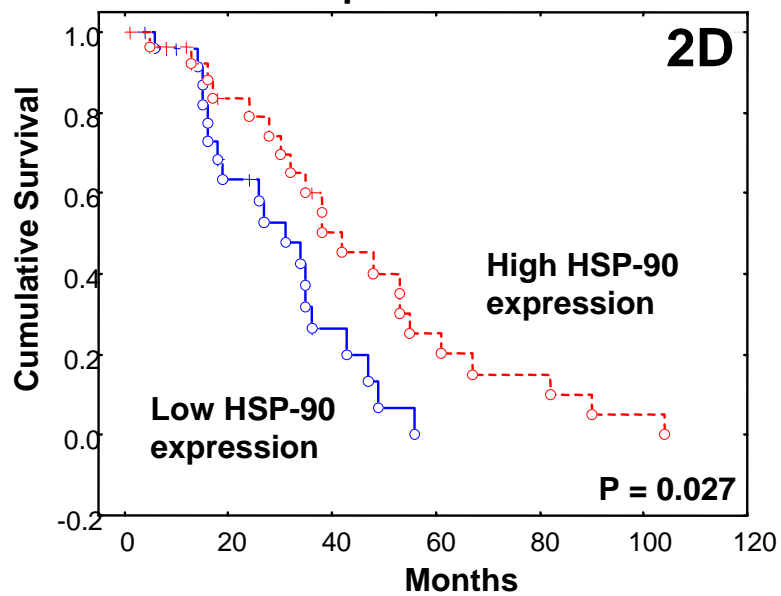
pM0 cases
