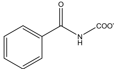
Hippurate
