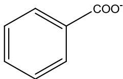
Benzoate
