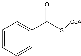
Benzoyl CoA
