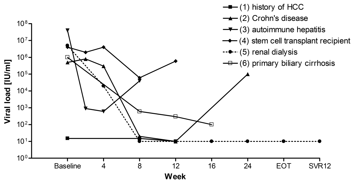
Additional figure 1. Individual courses of DAA experienced patients [A] and patients with special comorbidities [B]. Each line represents the viral load of one individual patient. Patients who have achieved SVR12 are represented by dotted lines. Figure legends identify medication and outcome of prior therapy, as well as the protease inhibitor
