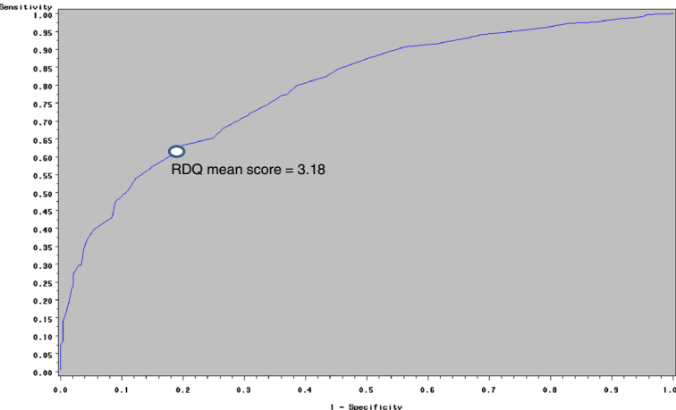
ROC Curve
