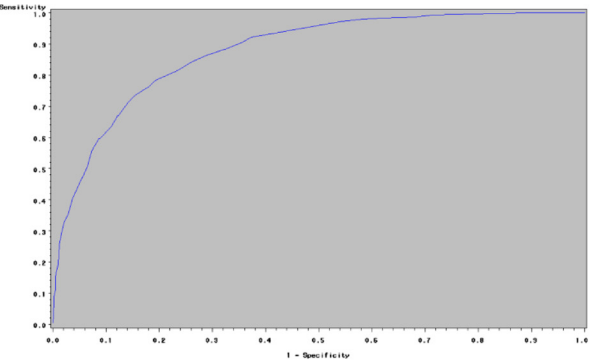
ROC Curve-Mild
