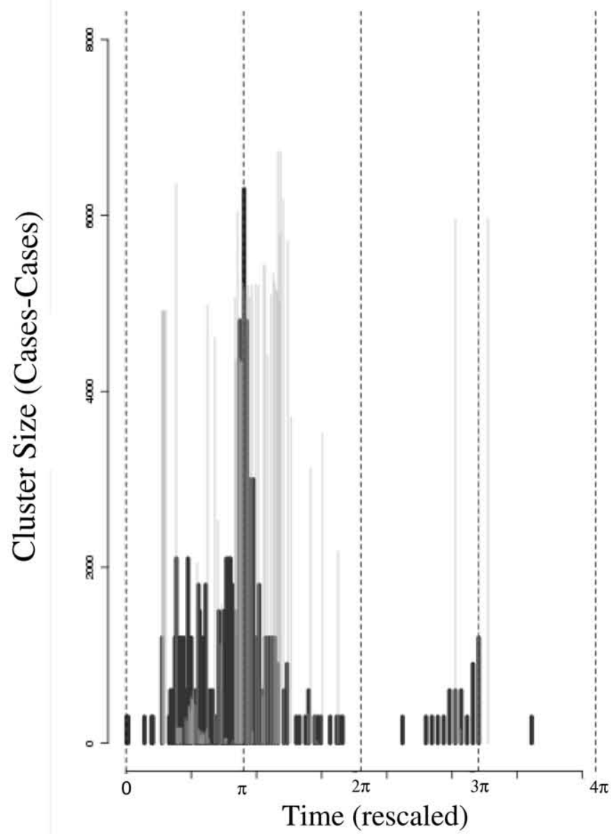
Classical Ogawa
