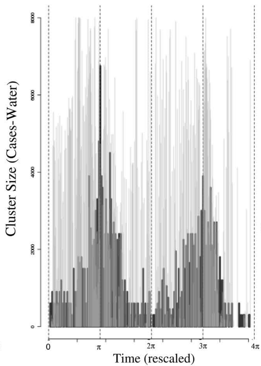
Classical Inaba
