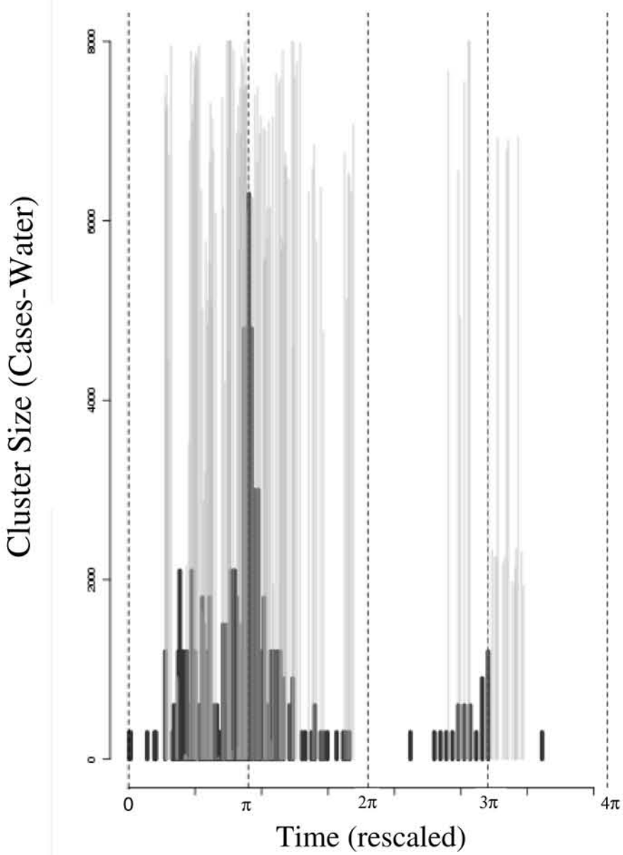
Classical Ogawa
