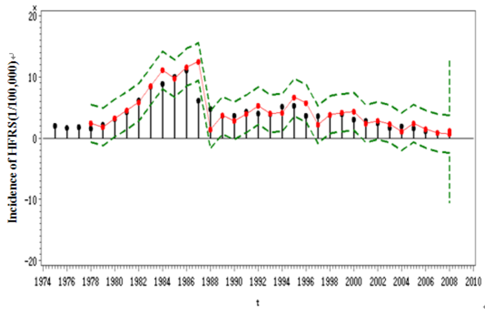
Figure 5 Black dots: observed values of HFERS incidence of China, for the period 1975-2008. Red solid line: ARIMA(0,3,1) model's fitted curve(1978-2008). Red dots: ARIMA(0,3,1) model's fitted values (1978-2008). Dashed lines: 95% confidence intervals of predicated values.
