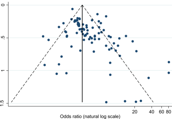
Funnel Plot
