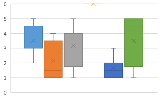
Consensus Ranking over Start-of-Flu-season - Region 10
