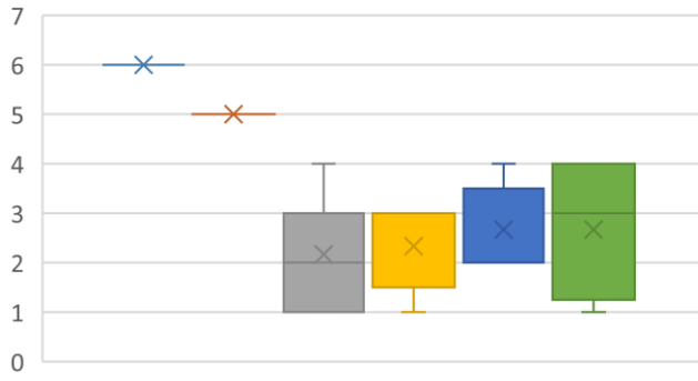
Consensus Ranking over Peak Value - Region 10
