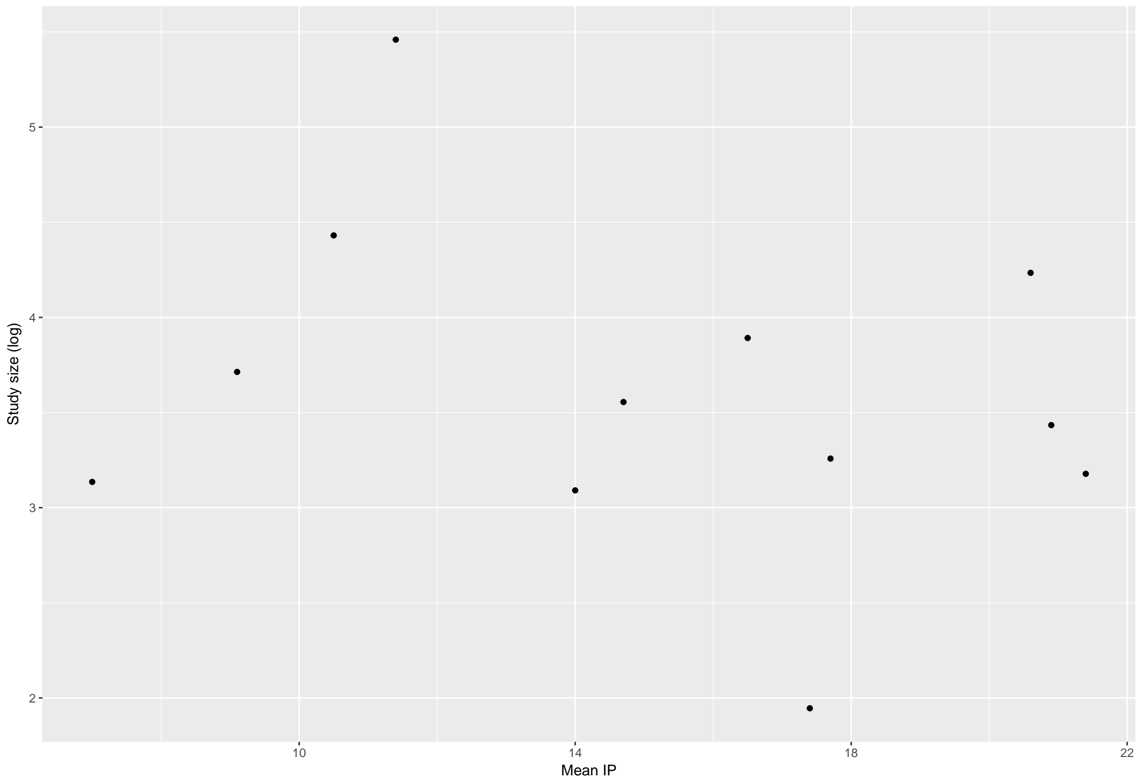
Funnel plot
