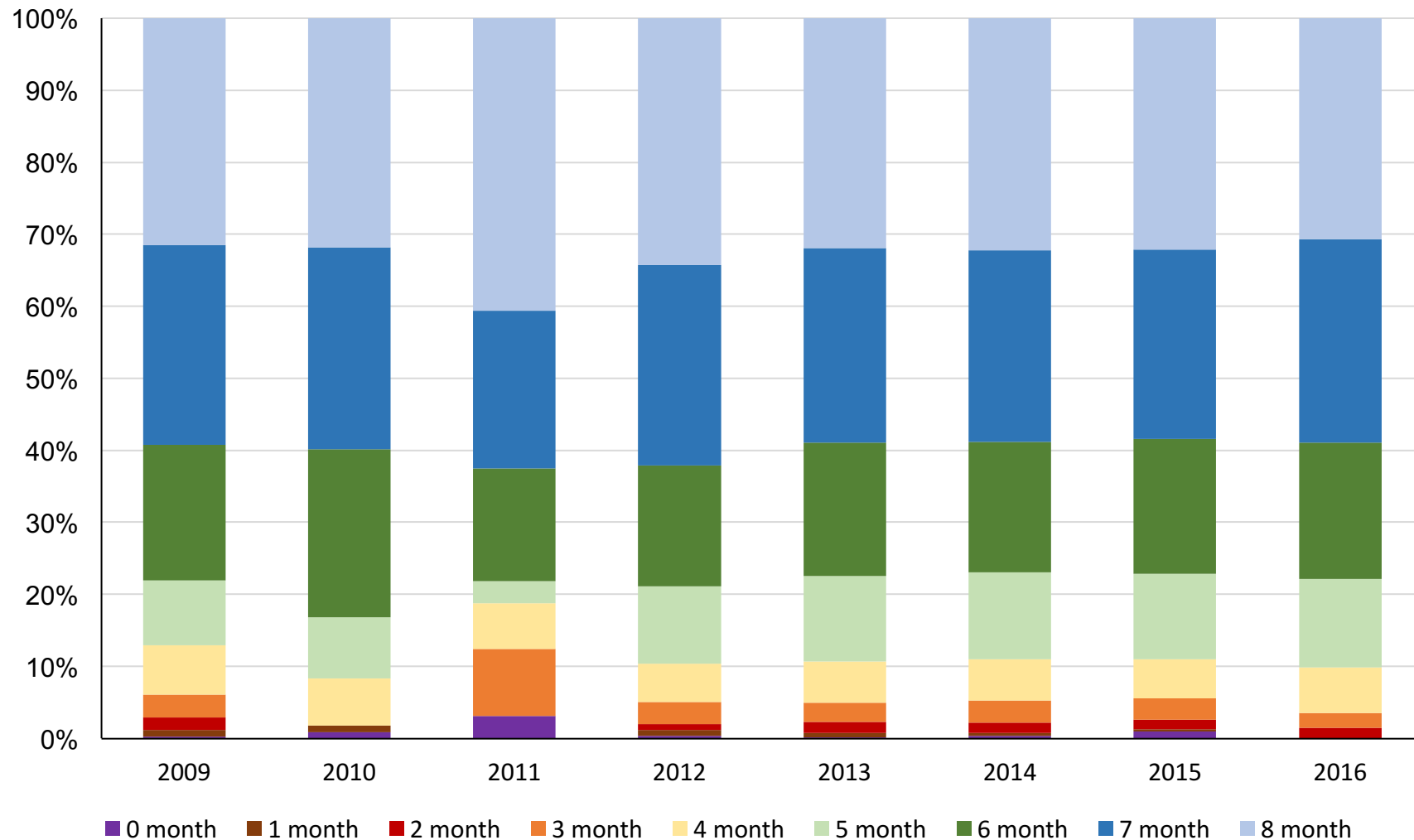
Figure S1. Distribution of measles cases by month-age among \leq 8 month old cases in each year
