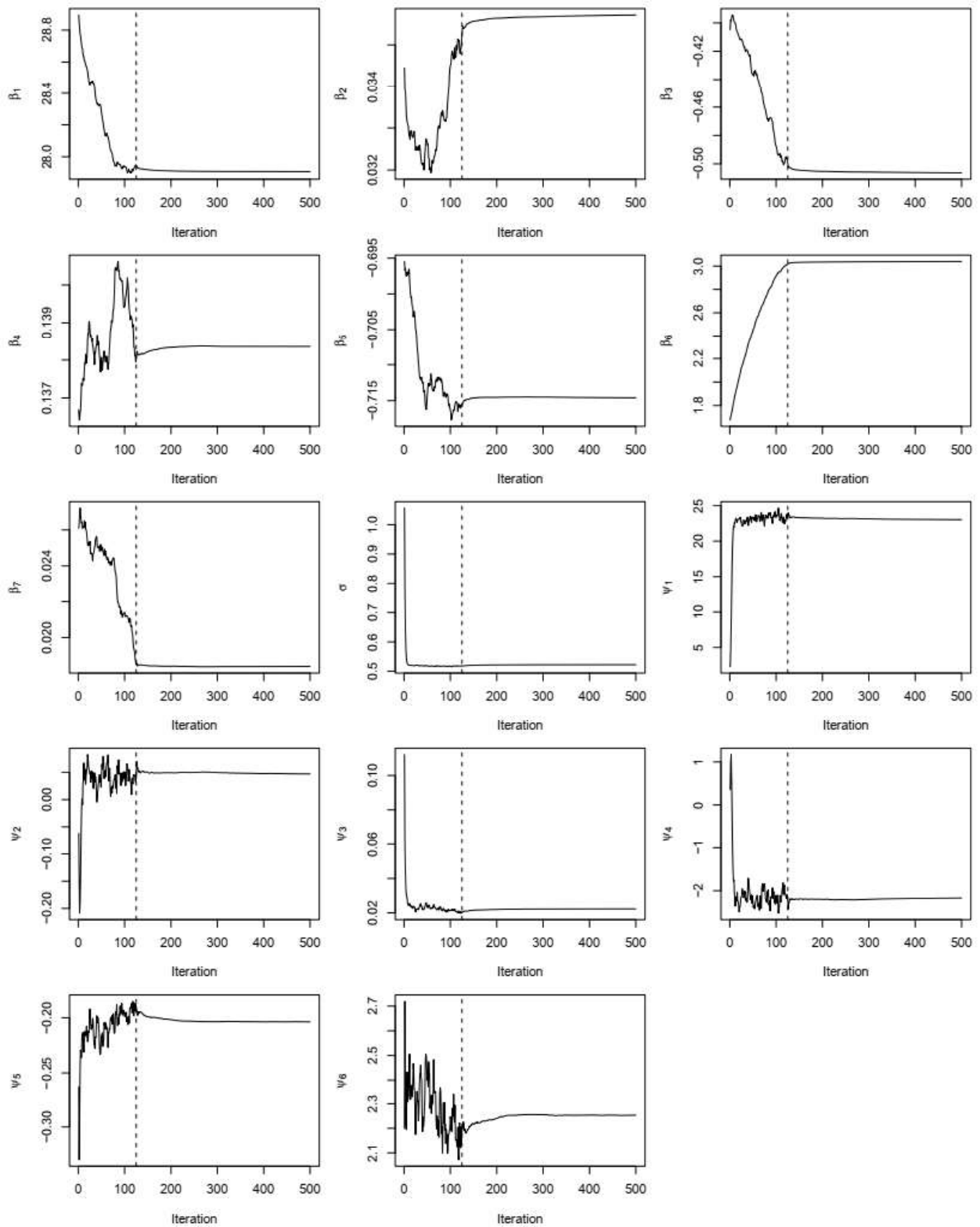
Convergence plots for quantile 0.85
