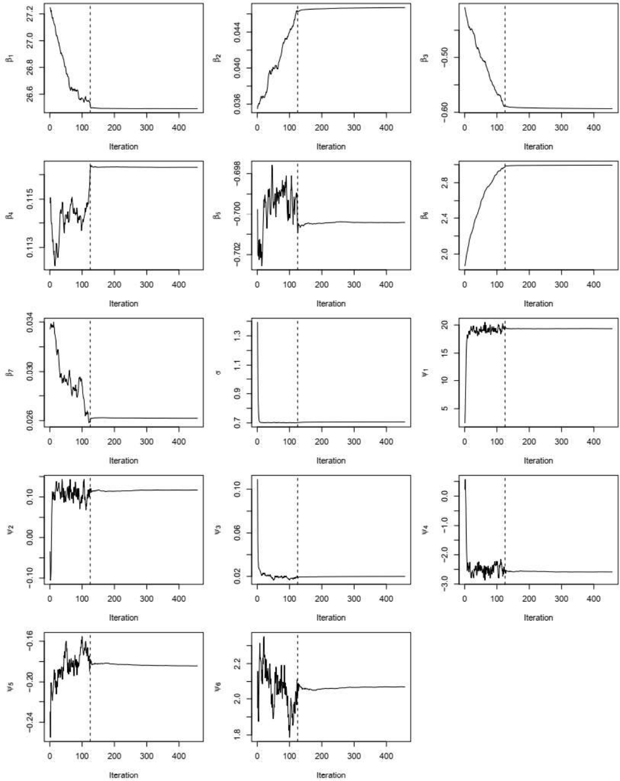
Convergence plots for quantile 0.75
