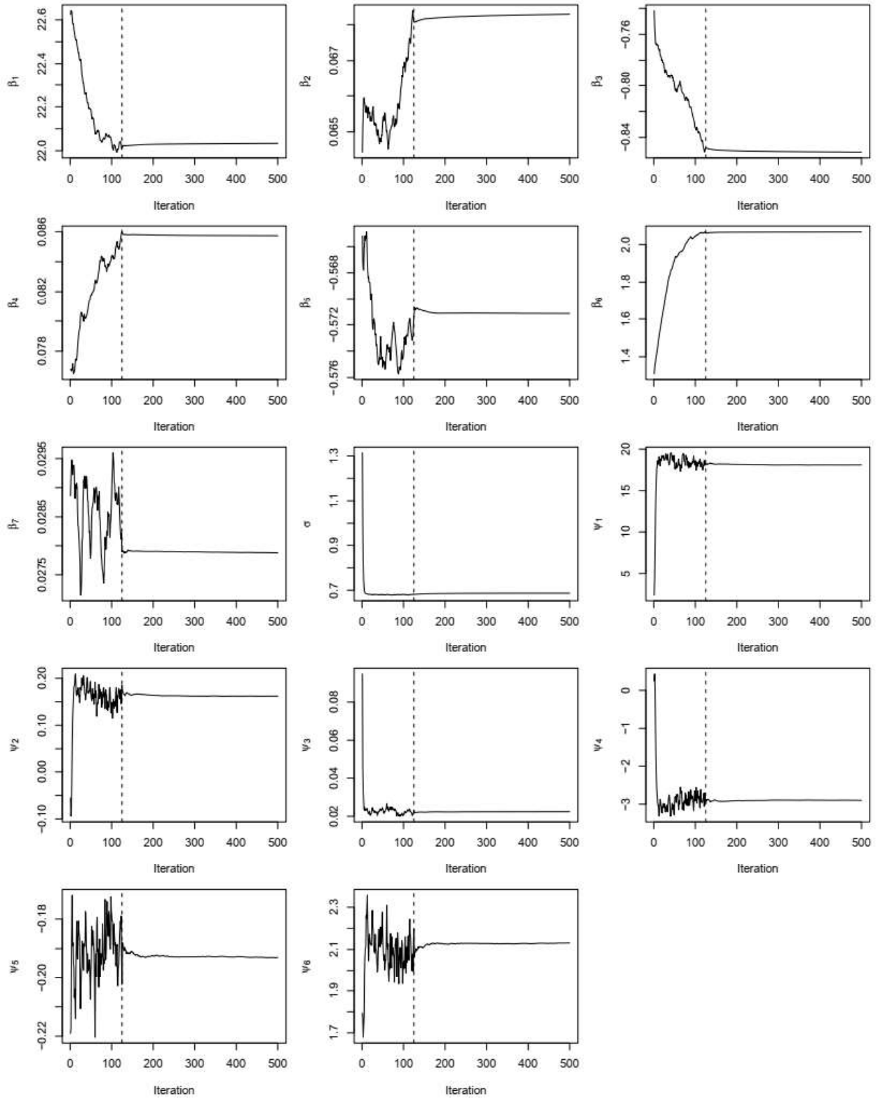
Convergence plots for quantile 0.25
