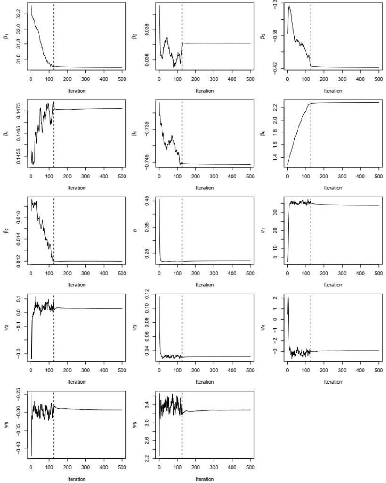
Convergence plots for quantile 0.95
