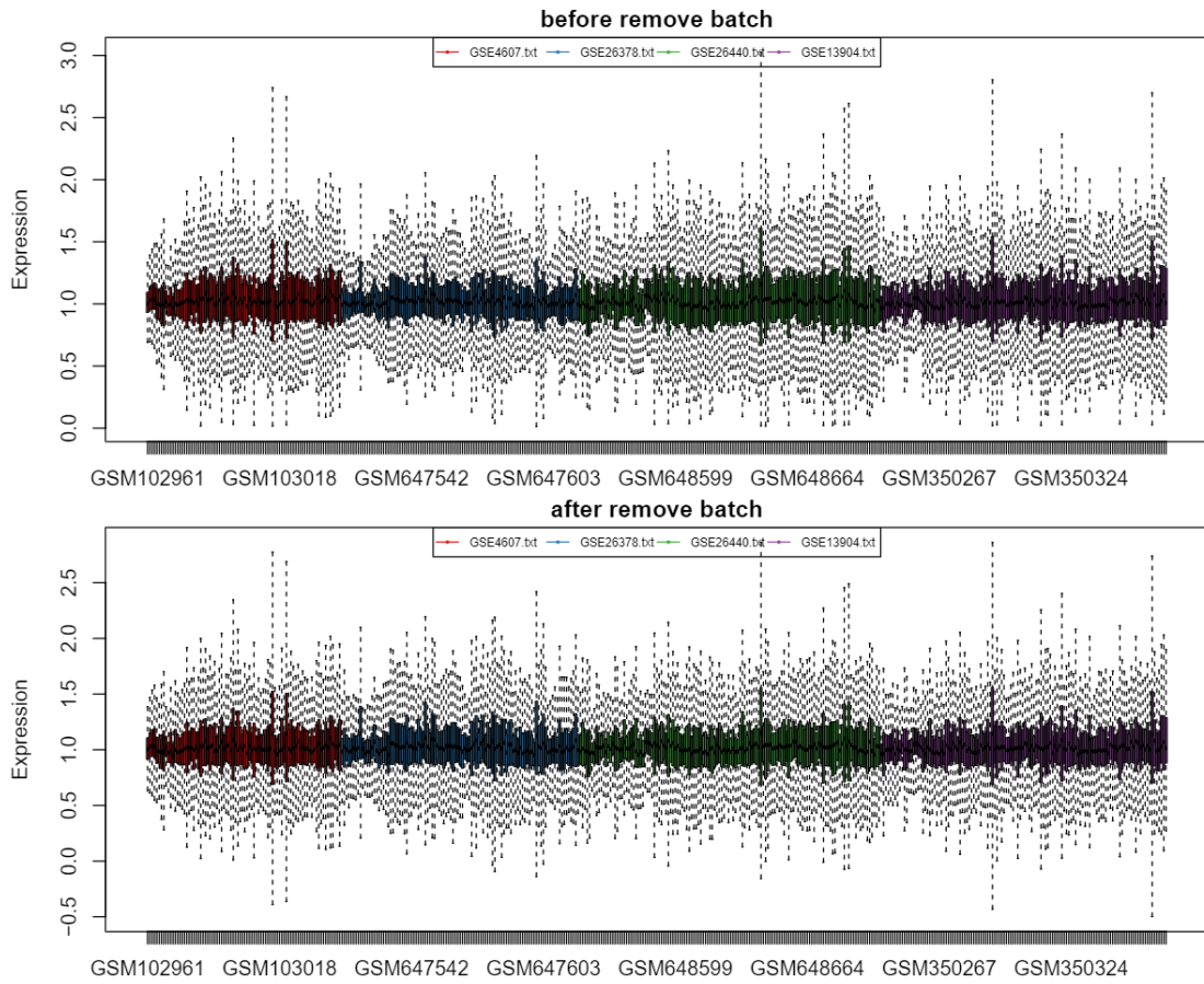
Figure S1 Batch effect processing between different data sets.
