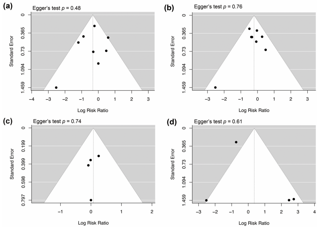
Figure S2. Funnel plots to assess publication bias for (a) SBP, (b) mortality, (c) incidence of overall infection, and (d) incidence of adverse events. SBP, spontaneous bacterial peritonitis.
