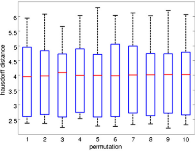
(a) Hausdorff
