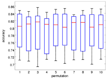
(c) Accuracy
