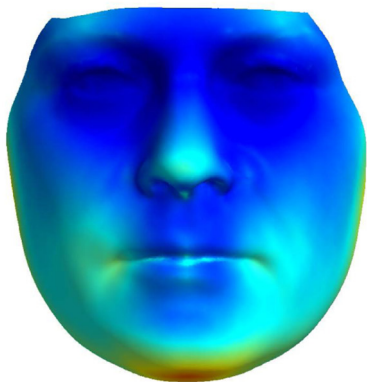
Landmark selections 2
