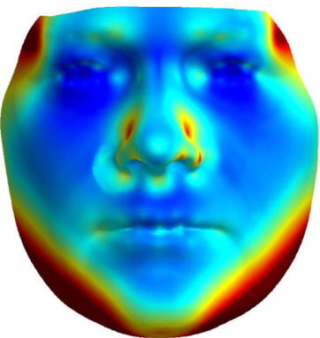
All points
