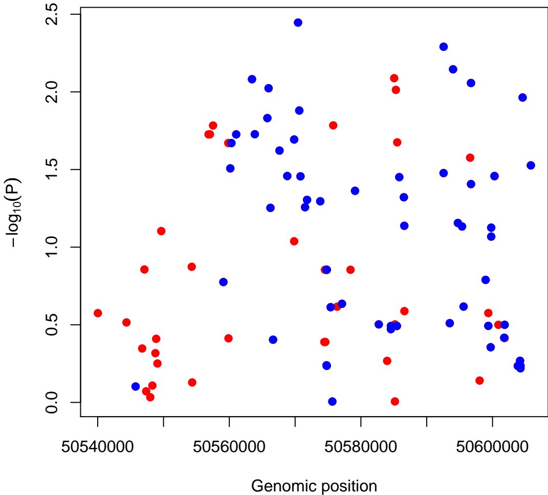
A) Single marker association scores
