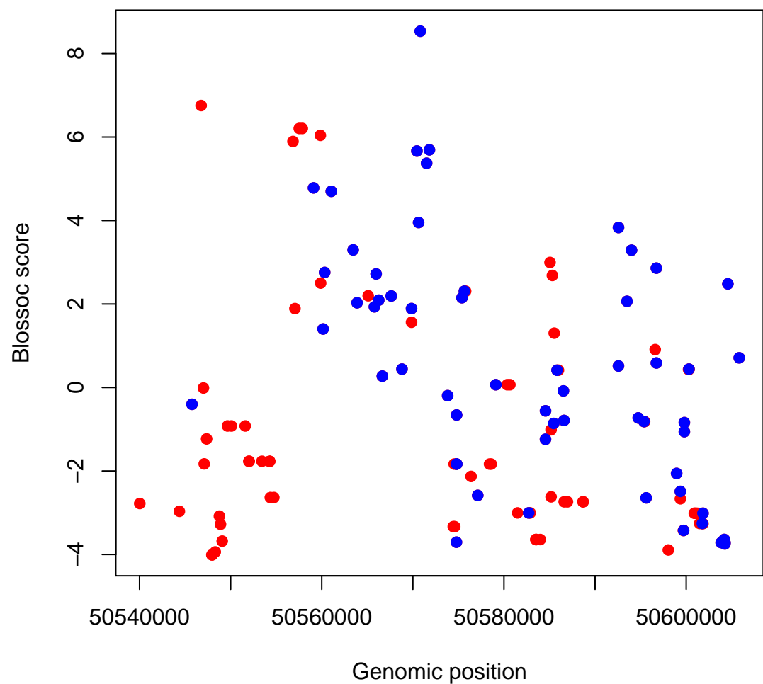
B) Blossoc association scores
