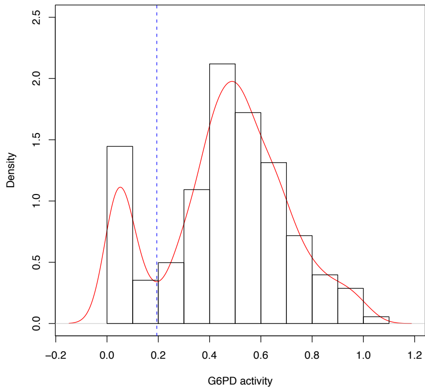
Figure S5. Defining qualitative G6PD deficiency. The intermodal minimum in the G6PD activity distribution in males was determined using kernel density estimation of the probability density function (red) and provided our ad hoc cutoff (blue) for distinguishing normal vs. deficient. A histogram of the G6PD activity distribution in males is superimposed for clarity.
