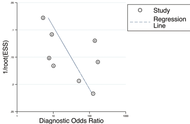
Deeks' Funnel Plot (uNGAL) P value = 0.12
