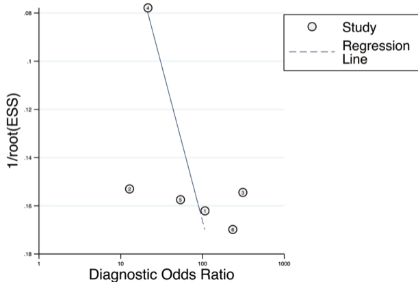
Deeks' Funnel Plot (bNGAL) P value = 0.16
